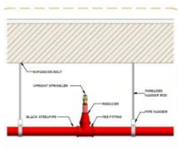
UPRIGHT SPRINKLER SECTION
