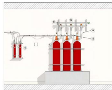
DETAILED SECTION 02
