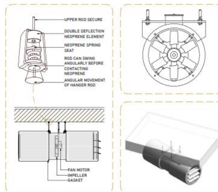
3D ISOMETRIC
