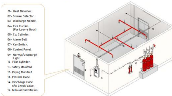
SYSTEM COMPONENT
